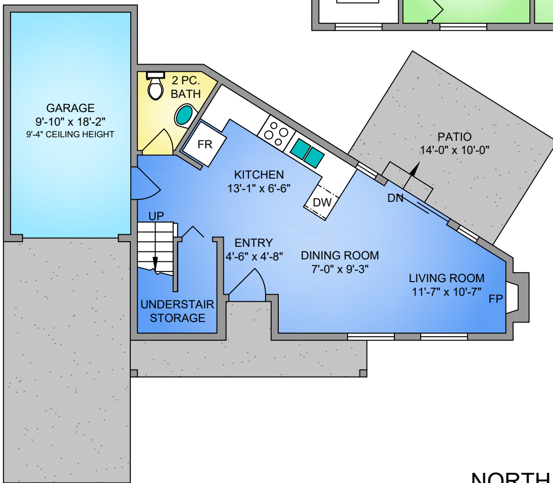
MAIN FLOOR 496 SQ. FT. 9'-0" CEILING HEIGHT
