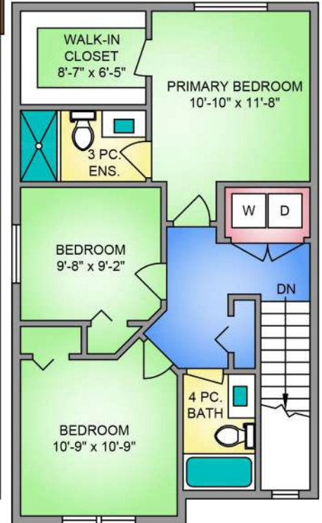
THIRD FLOOR 736 SQ. FT. 8'-0" CEILING HEIGHT
